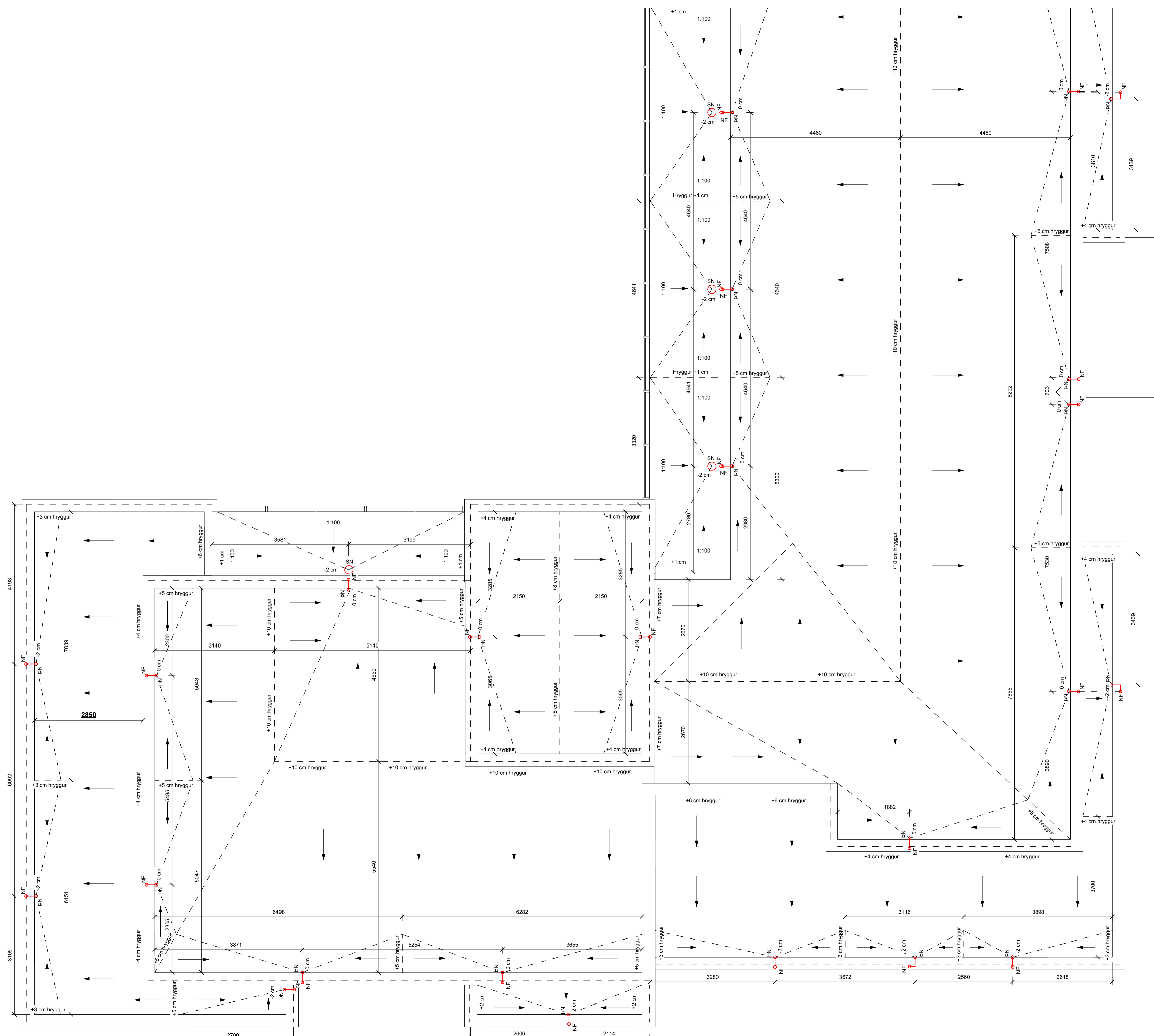
ÞAKHALLAPLAN - B mkv: 1 : 50
