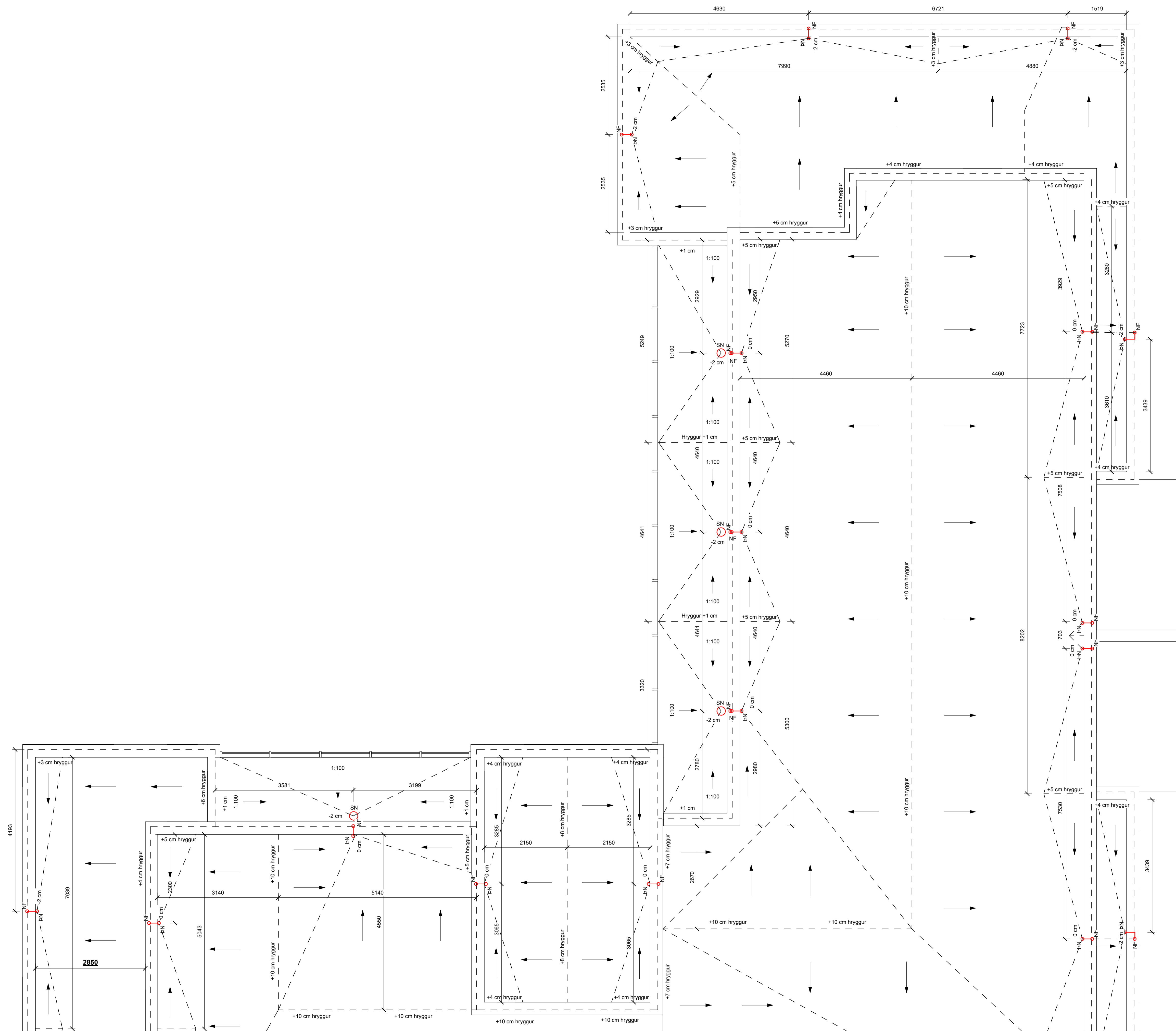
ÞAKHALLAPLAN - A mkv: 1 : 50
